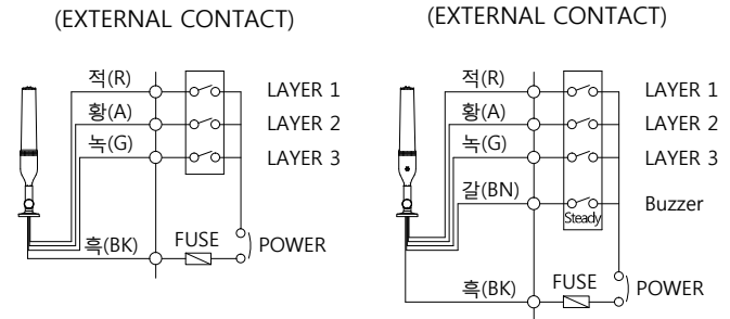
ELECTRICAL CONNECTION DIAGRAM
