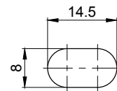
FITTING HOLES
